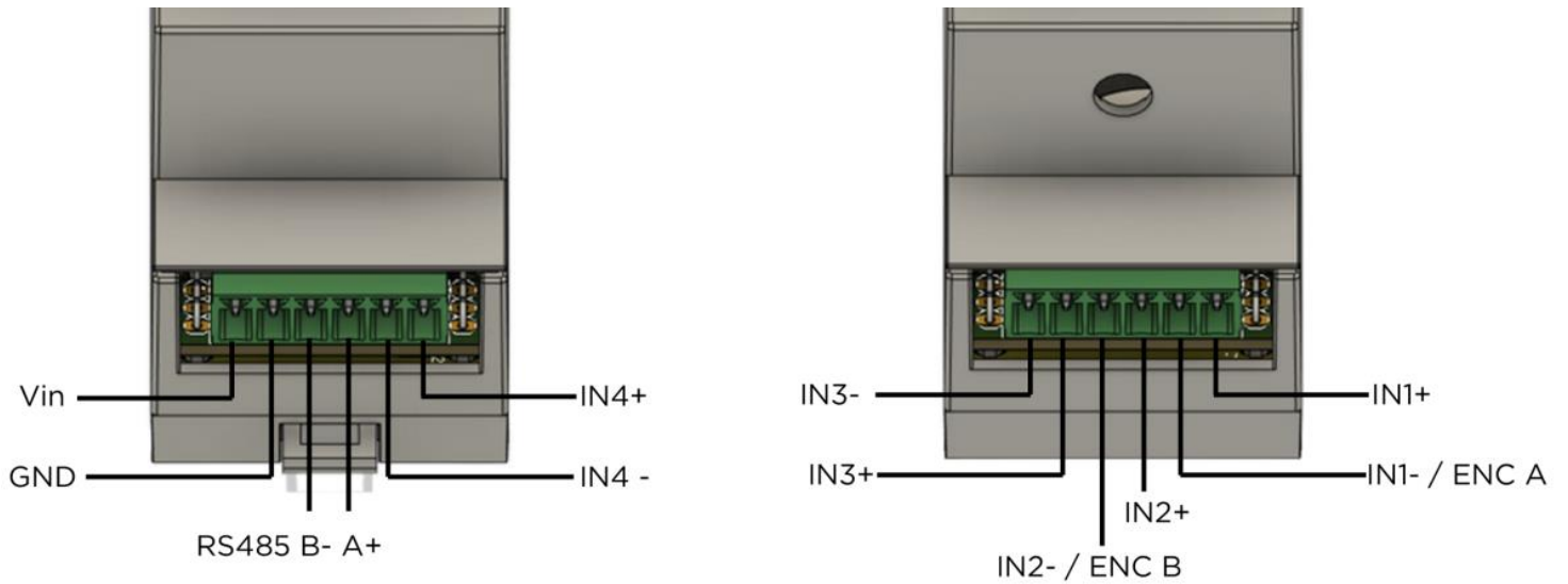
Illustration 2 - Lower and upper side connectors
